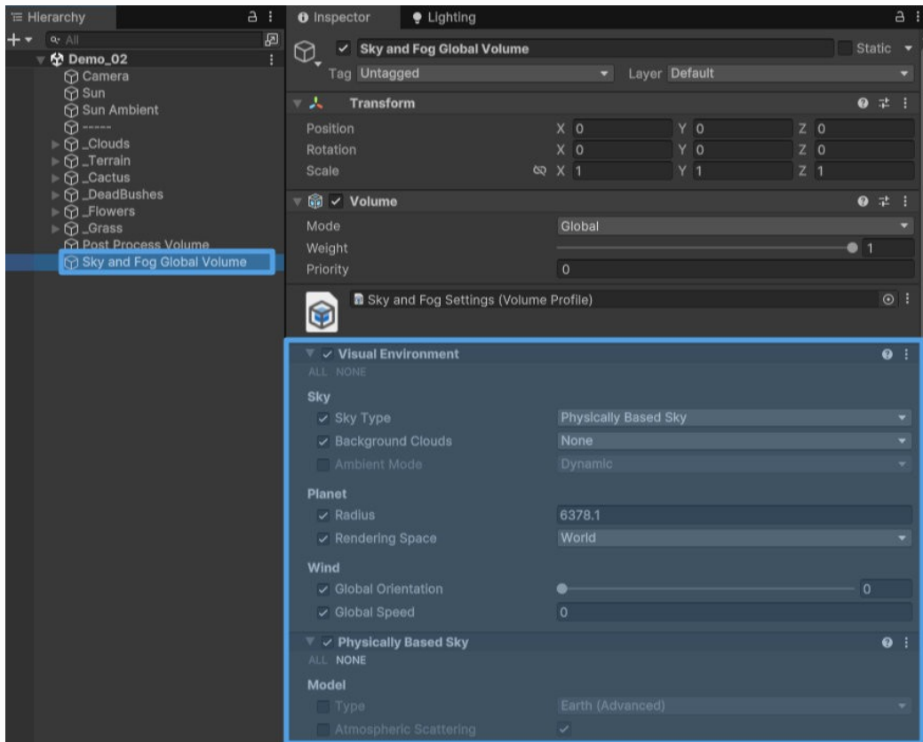
Unity 6 example
