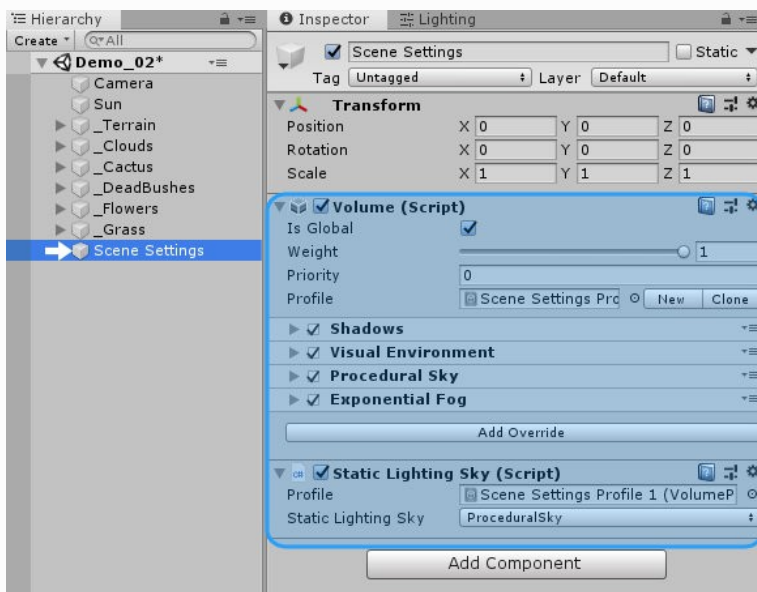
Unity 2019.4 example
